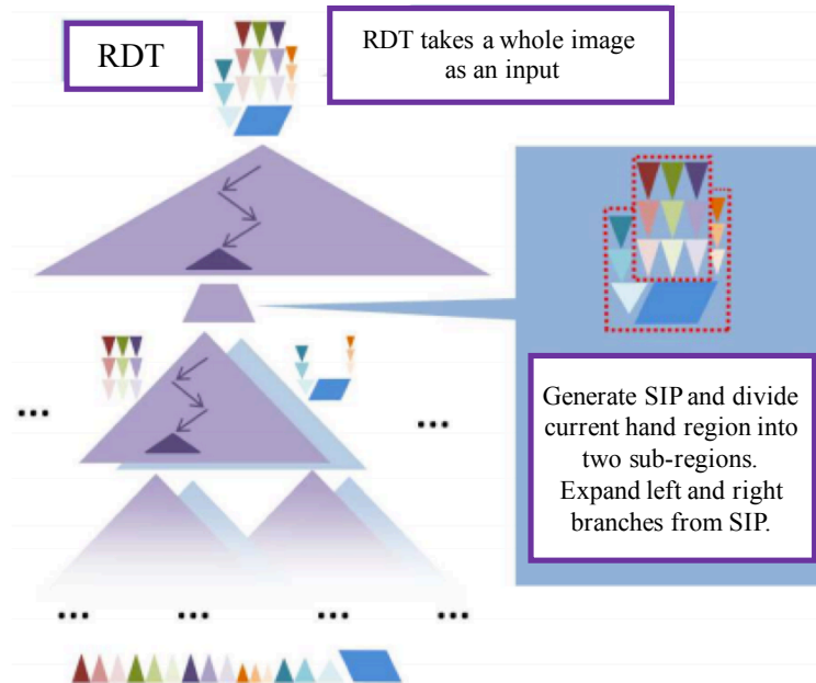
Figure 19 – Growing a Random Decision Tree (RDT) with Segmentation Index Points (SIPs), proposed by Li et al. [225]. Unlike in the previous case of LTM [289], where the model was learned in advance and kept fixed , here the training objectives (SIPs) are adaptively estimated for each split.
